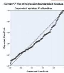
Gambar 1. Grafik Normal Plot
